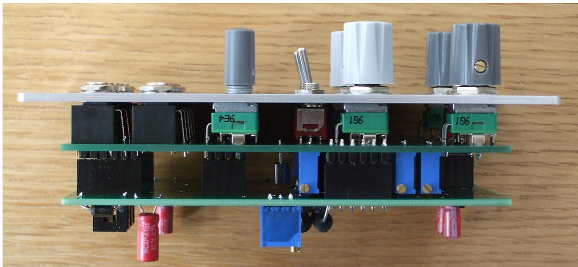
The completed module from the side. Note firstly the side adjust trimmers that allow the trimming to be done from the side of the module, and secondly that the pots with the micro control knobs do not have any mounting nuts and washer fitted.
