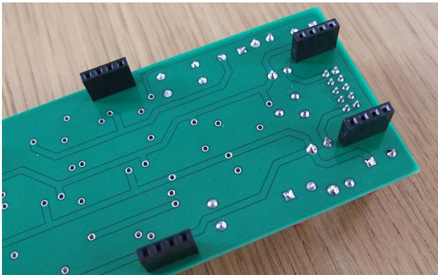
This is the underside of the Oakley COTA filter module's main board but the DVCO main board has its SIL sockets mounted in a similar way.
