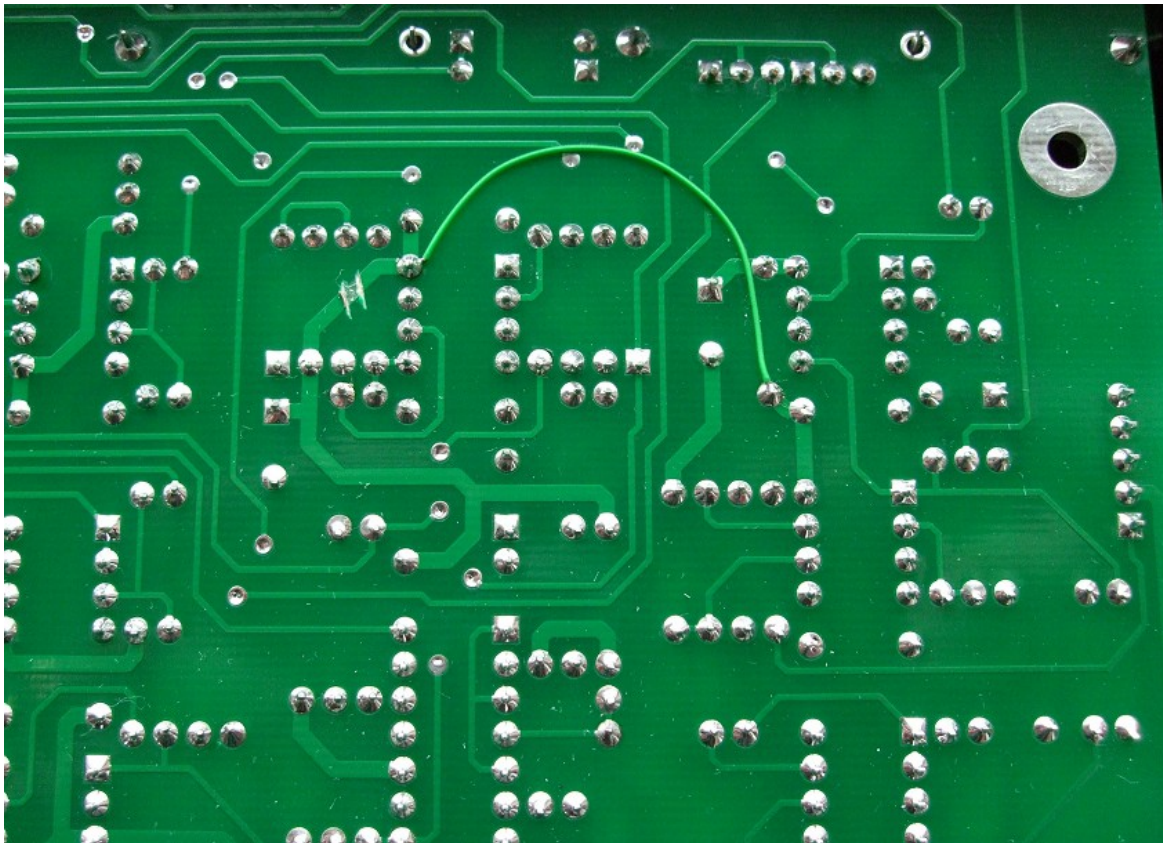
A close up of the underside of the issue 3 board. Issue 3.1 & 3.2 boards do not need to be modified.
