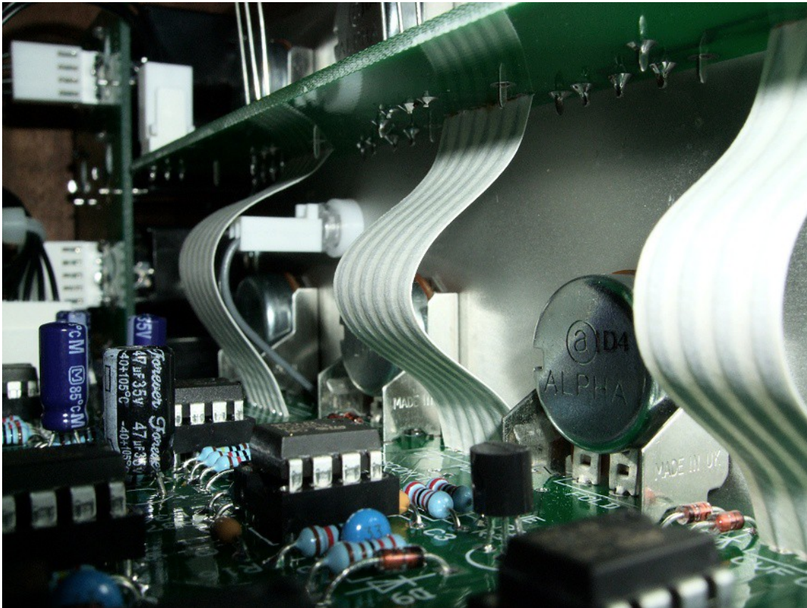
Close up of the pot board to main board interconnects and the LED connection. Here I have used my usual method of a two way Molex KK to attach the LED to two fly wires from the main board.
