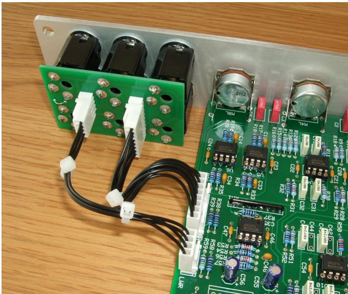
The Sock6 board makes it much easier to build the module. Here I have used Molex 0.1" KK headers and housings. This is a 'strip and crimp' system that is cheap but very reliable.
