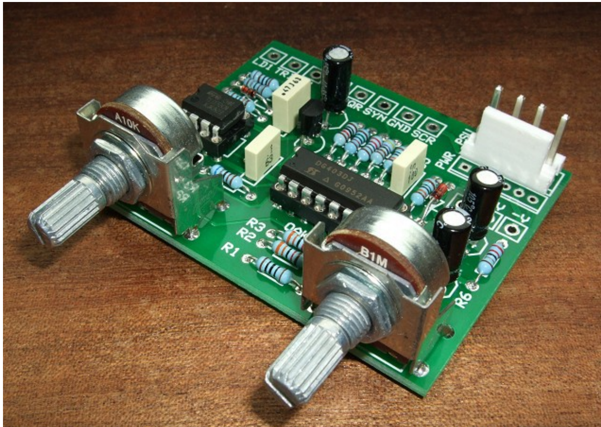
The issue 6 Little-LFO board fully populated. The MTA156 header has been fitted to this one allowing it to connect to the Oakley/MOTM and Fractional Rack modular systems. The pots used here are the ones with a short 6mm knurled shaft.
