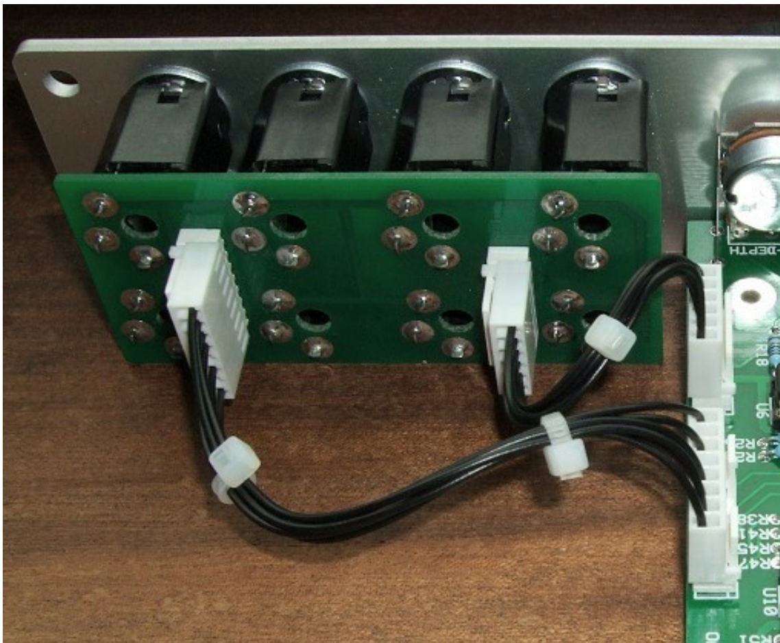
Both board interconnects made up and cable tied into place for neatness. This is the cheaper but perfectly decent Molex KK 0.1" header system.
